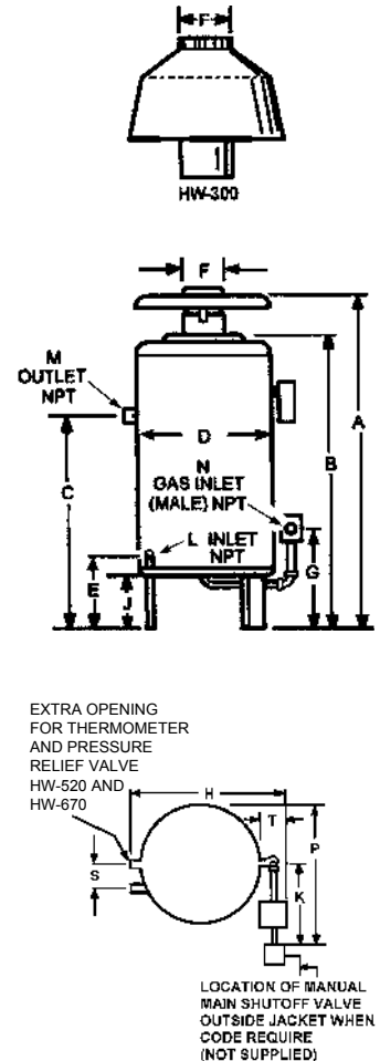
FIGURE 1. DIMENSIONS
