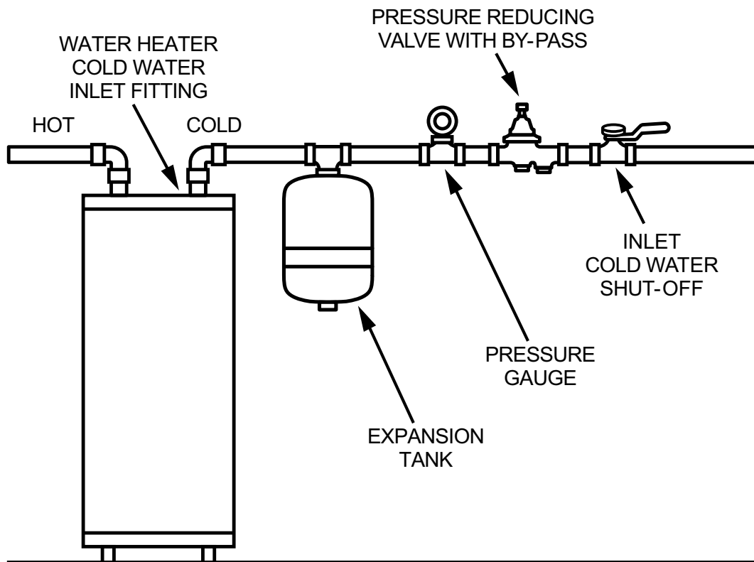
RECOMMENDED INSTALLATION - VERTICAL MOUNTING
