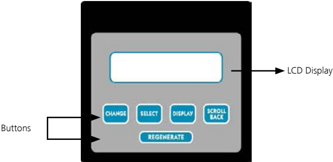
Diagram 18: Five-Button Controller
