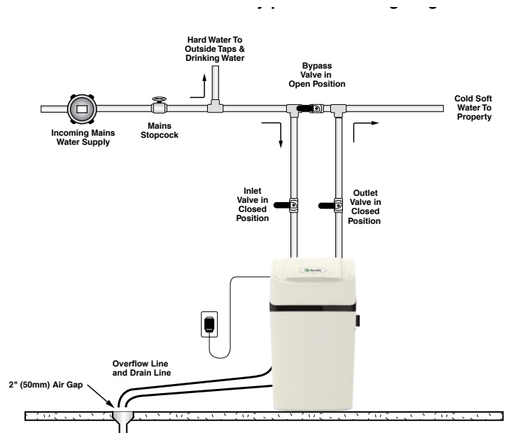
Diagram 11: Bypass Position
