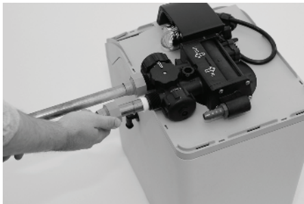
Diagram 9: Connect Water Lines (Shown with Bypass Valve)
