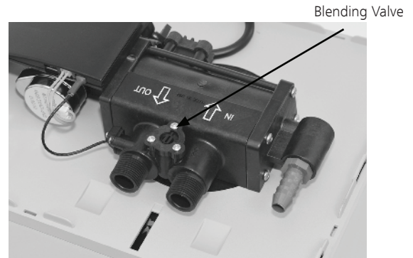
Diagram 18: Adjusting Blending Valve
