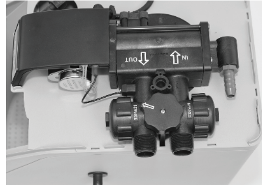
Diagram 17: Bypass Valve
