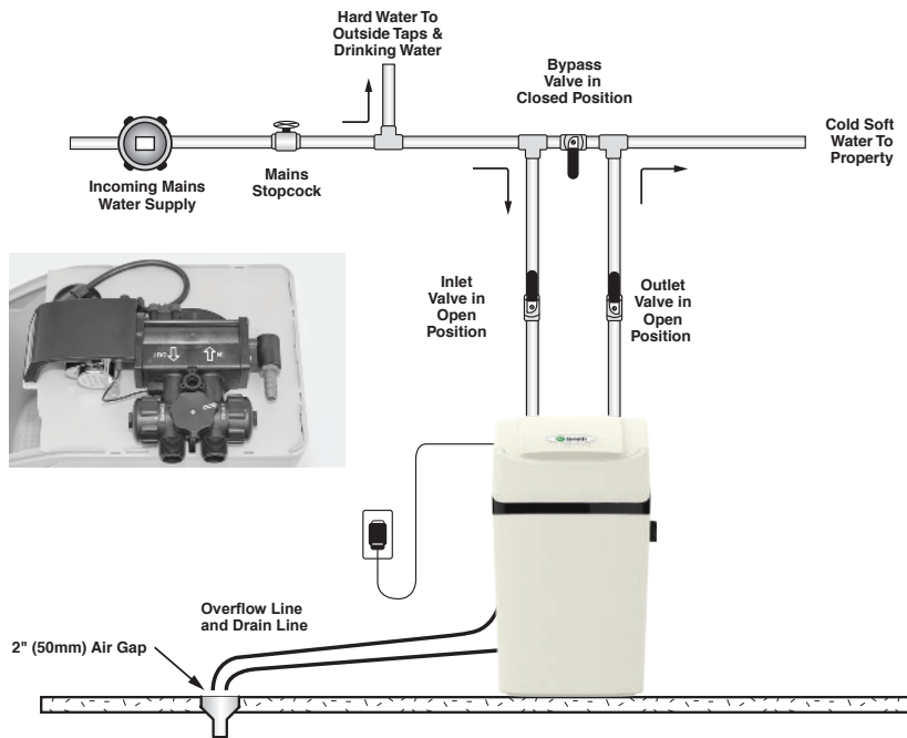
Diagram 13: Service Position
